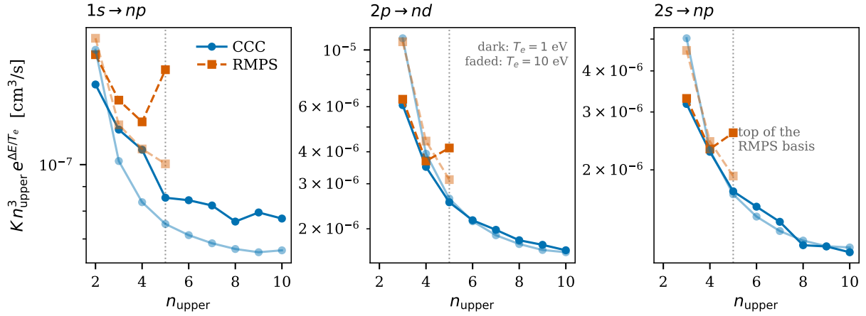
Figure 2.3: Which of the two calculations is anomalous at n = 5 . The reduced rate coefficient Kn_{\text{upper}}^3 e^{\Delta E/T_e} of Eq. (2.12) along three dipole series, with the threshold factor the two calculations share divided out. For hydrogen the oscillator strength falls as n_{\text{upper}}^{-3} asymptotically, so this quantity must flatten as the series is climbed; the constant it approaches is not used, only the smoothness. Dark curves are T_e = 1 eV, faded curves 10 eV. CCC continues to n = 10 . At 1 eV the RMPS values track CCC to n = 4 and then rise into n = 5 , the top shell of their target basis, in all three series; at 10 eV neither calculation kinks and the RMPS values are uniformly the flatter. The kink belongs to the temperatures at which the Maxwell average samples the cross section close to the n = 5 threshold. It localises the departure from hydrogenic behaviour at one shell of one calculation without proving CCC correct, which is not smooth there either. From anderson_validity_dipole_series.csv , columns R_CCC_bz and R_And_bz .
