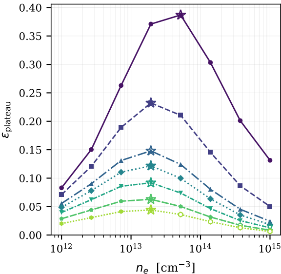
(a) heating, +5% step in T_e ; all 8 columns
