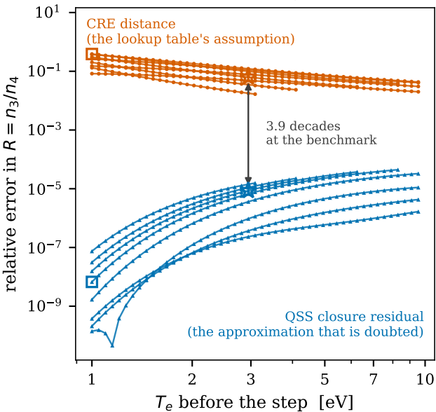
(a) both errors, all 8 density columns
