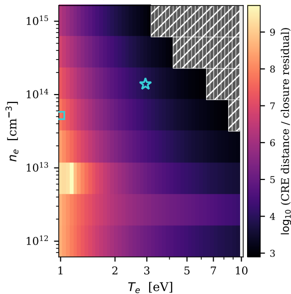
(b) the gap, over the grid
