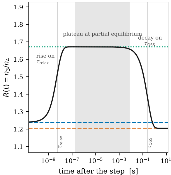
(b) coldest grid point: T_e 1.00 \rightarrow 1.05 eV, n_e = 5.2 \times 10^{13} \text{ cm}^{-3}
