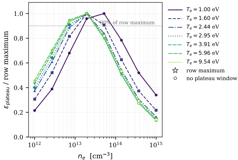
(b) each row divided by its own maximum
