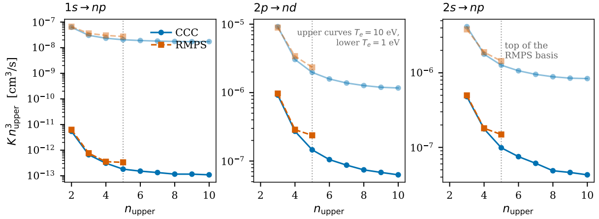
Figure 2.3: Which of the two calculations is anomalous at n = 5 . The reduced rate coefficient K n_{\text{upper}}^3 along three dipole series. For hydrogen the oscillator strength falls as n_{\text{upper}}^{-3} asymptotically, so above threshold this quantity must flatten as the series is climbed; the constant it approaches is not used, only the smoothness. Dark curves are T_e = 1 eV, faded curves 10 eV. CCC continues smoothly to n = 10 . The RMPS values track it until the step into n = 5 , the top shell of their target basis, where all three series flatten early – the signature of a truncated close-coupling expansion accumulating in its highest physical shell flux that belongs to n \geq 6 and the continuum. This localises the departure from hydrogenic behaviour at one shell of one calculation. It does not prove CCC correct: the scaling is asymptotic and weakest at 1 eV, which is where the kink is largest. From anderson_validity_dipole_series.csv .
