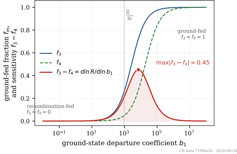
Figure 3.4: The ground-fed fractions of the two shells and their difference, at the benchmark point; the dotted vertical line marks b_1^{\text{CRE}} there. Both fractions rise from zero to unity as the ground-state reservoir grows, but they do so at different rates, and their difference, which by Eq. (3.39) is exactly d \ln R / d \ln b_1 , vanishes in both limits and peaks where the two supplies compete. Note that f_3 - f_4 is a difference of fractions, not itself a fraction.
