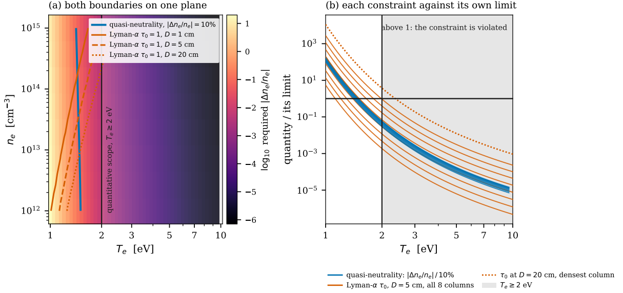
Figure 5.8: Two independent constraints put the same floor under the quantitative scope. Both boundaries are measured contours at thresholds that were chosen, 10% for the density change and \tau_0 = 1 for the optical depth, and they come from unrelated physics. Quasi-neutrality. Imposing nuclei conservation across one grid step in T_e , the electron density must change by |\Delta n_e/n_e| = |\Delta n_g|/n_{\text{ion}} , taken from the two CR-equilibrium solves either side of the step. This zero-dimensional model holds n_e fixed, so wherever that requirement is large the model is contradicting itself. Of the 392 one-step operators on the grid, 68 require more than 10% and 36 require more than 100%. At T_e = 1 eV the fixed-density inference gives 10.1 to 20.0; solved self-consistently for a closed parcel the density rises by a factor 1.98 to 2.05, and the counts become 67 and 7 ( validation/closed_nuclei/ ). At T_e \geq 2 eV it never exceeds 0.0054. The 10% contour sits at T_e = 1.41 to 1.50 eV and is almost independent of density. Optical depth. The Lyman- \alpha line-centre optical depth over the half slab, \tau_0 = n(1s) \sigma_0 D/2 , with \sigma_0 evaluated at T_{\text{at}} = T_e from the Doppler width \sqrt{2kT/m} , giving \sigma_0 = 5.474 \times 10^{-14} \text{ cm}^2 at 1 eV. The optically thin matrix used throughout this thesis is only defensible where \tau_0 < 1 . That contour runs from T_e = 1.13 to 1.98 eV at the slab thickness D = 5 cm, and across the 3 thicknesses in the trapping sweep it spans 1.01 to 2.36 eV. (a) Both boundaries on the (T_e, n_e) plane, over a map of the quasi-neutrality requirement. (b) Each constraint divided by its own limit, so that a value above one means the constraint is violated and the two can share a single axis. Both boundaries fall between 1.01 and 2.36 eV. Two independent pieces of physics, particle conservation and radiation transport, place the floor in the same narrow band, and T_e \geq 2 eV clears both everywhere except 2 of the 3 times eight optical-depth crossings, which sit at the largest slab thickness D = 20 cm and the two highest density columns. The T_e \geq 2 eV restriction is therefore a measured boundary, not a hedge.
