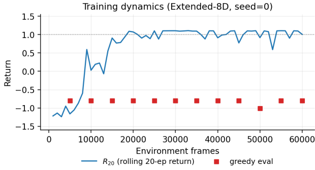
Fig. 3: Training dynamics on the 7 \times 7 grid world (60,000 frames, seed = 0). The 20-episode rolling return R_{20} stabilises around +1.0 after \sim 15k frames; periodic greedy evaluations are overlaid as squares.
