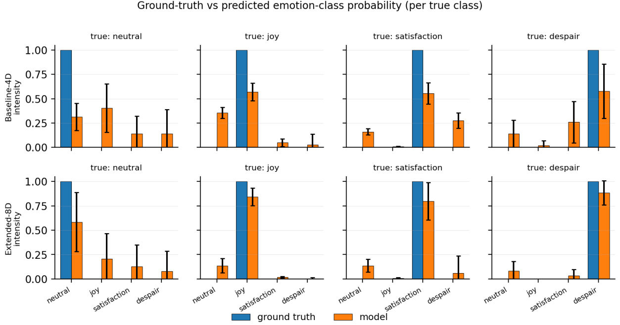
Fig. 8: Per-class probability calibration on the held-out test set, in the per-class reporting style of [16] (Figs. 4–7). Each cluster shows the model’s mean predicted probability across the four emotion classes (orange, with \pm one standard deviation whiskers) for held-out instances whose true label is given in the panel title; the ground-truth one-hot intensity is overlaid in blue for reference. The Extended-8D model produces a substantially sharper diagonal profile than the Baseline-4D model.
