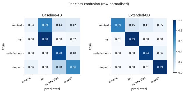
Fig. 9: Row-normalised confusion matrices on the held-out test set. The four-dimensional vector confounds neutral with joy and despair with satisfaction ; the eight-dimensional vector resolves both confusions.
