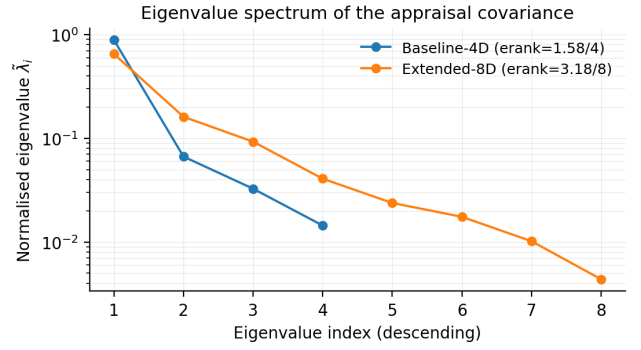
Fig. 2: Normalised eigenvalues \tilde{\lambda}_i of the appraisal covariance for both runs. The Baseline-4D spectrum collapses sharply onto its first eigenvector, leaving an effective rank of 1.58/4. The Extended-8D spectrum spreads mass over a longer tail, attaining an effective rank of 3.18/8.
