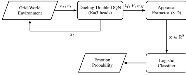
Fig. 1: End-to-end pipeline. The dueling Double DQN exposes Q , V and the cross-head standard deviation \sigma_K , all of which are consumed by the eight-dimensional appraisal extractor.
