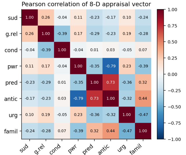
Fig. 4: Pearson correlation matrix of the eight appraisal dimensions over 60,000 frames. The largest world-driven off-diagonal entry, |r| = 0.79 between power and anticipation, is discussed in Section IX.
