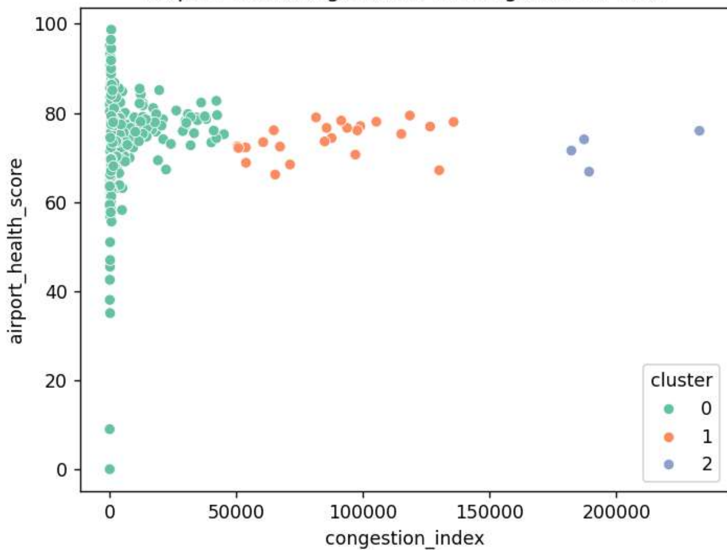
Airport Clustering: Stable vs Congested vs Risk
