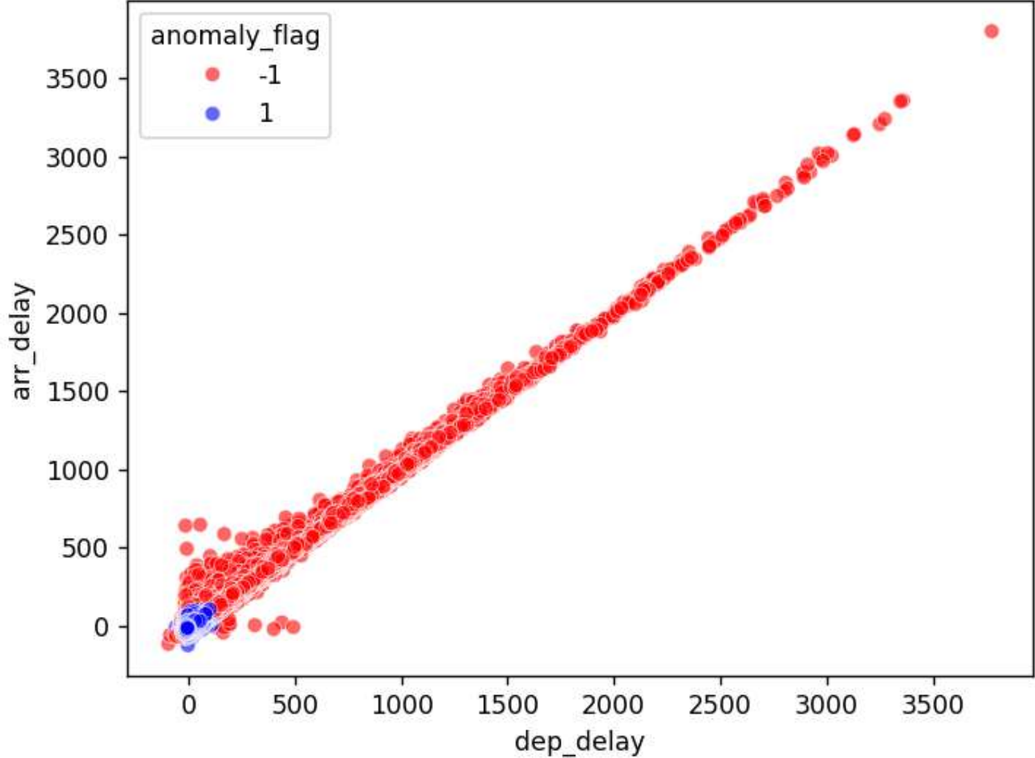
Anomaly Detection: Delay Spikes & Operational Issues
