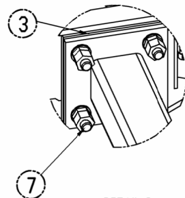
DETAIL B SCALE 1 : 10 BRACKET EXAMPLE
