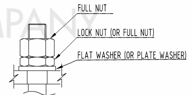
LOCK NUT INSTALLATION METHOD
