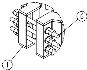
DETAIL B SCALE 1 : 10 BRACKET EXAMPLE
