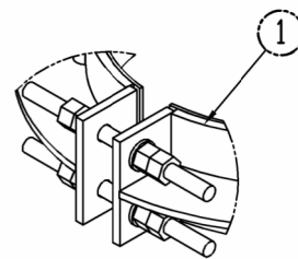
DETAIL B SCALE 1 : 10 COLLAR EXAMPLE
