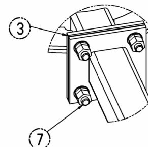
DETAIL B SCALE 1 : 10 COLLAR EXAMPLE
