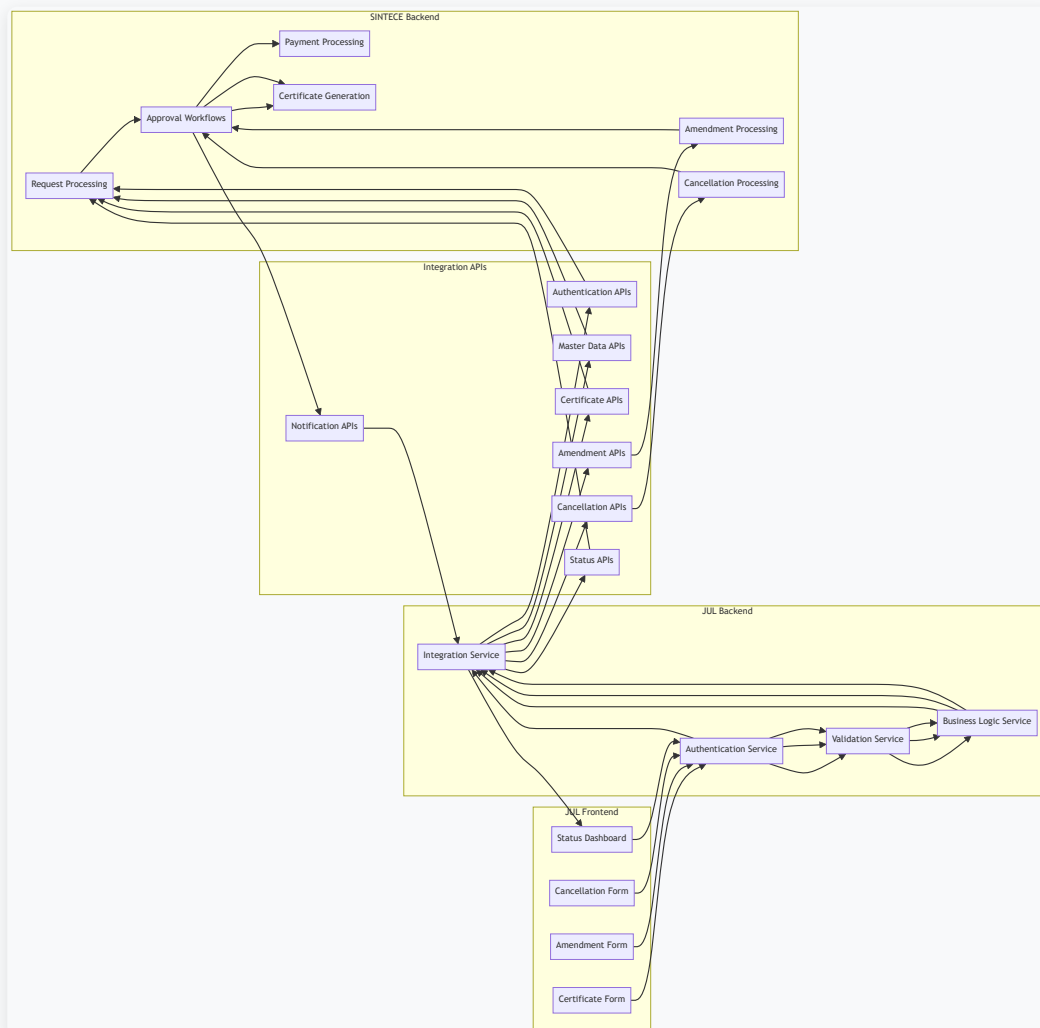
Figure 3.3: Integration API Flow Architecture
