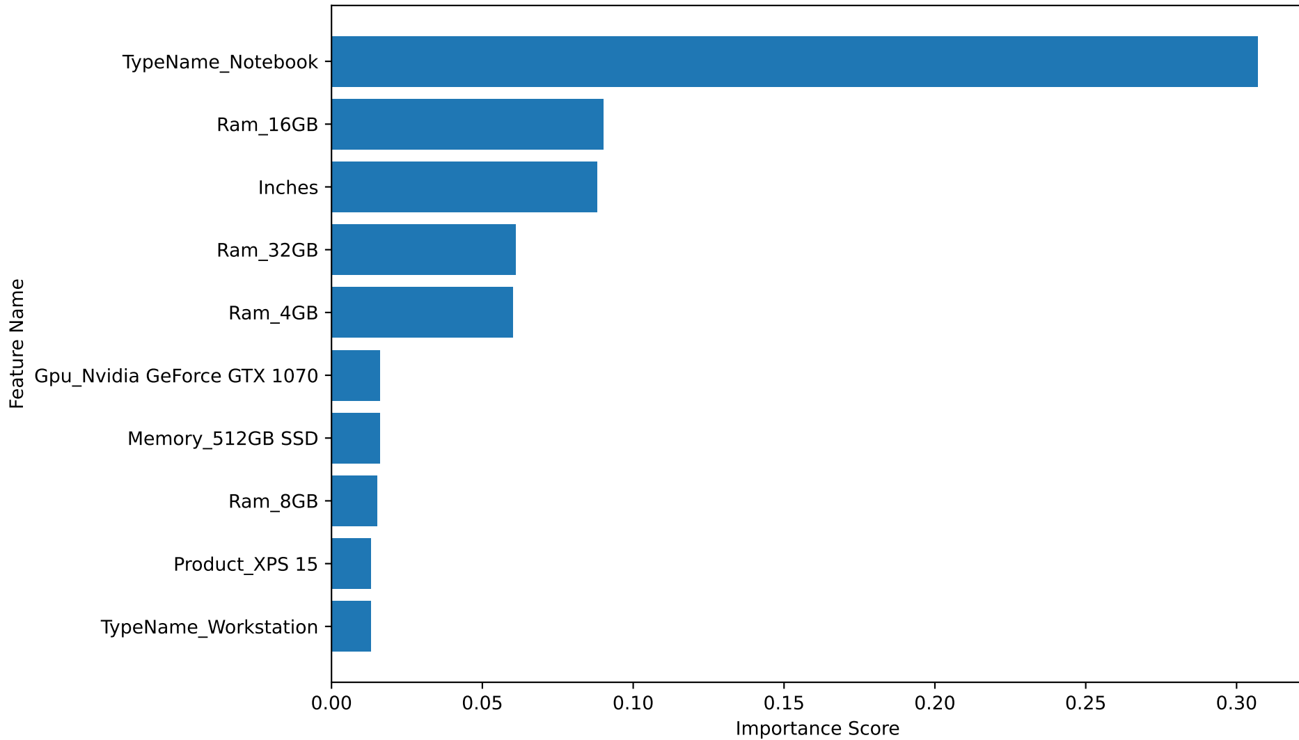
Figure 4: Feature Importance
