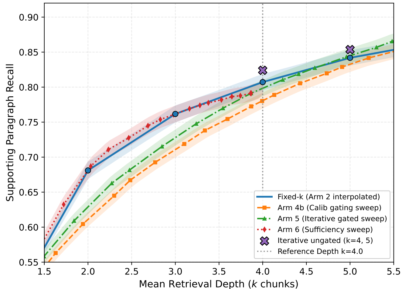
Bridge Multi-Hop Questions (N=2077)
