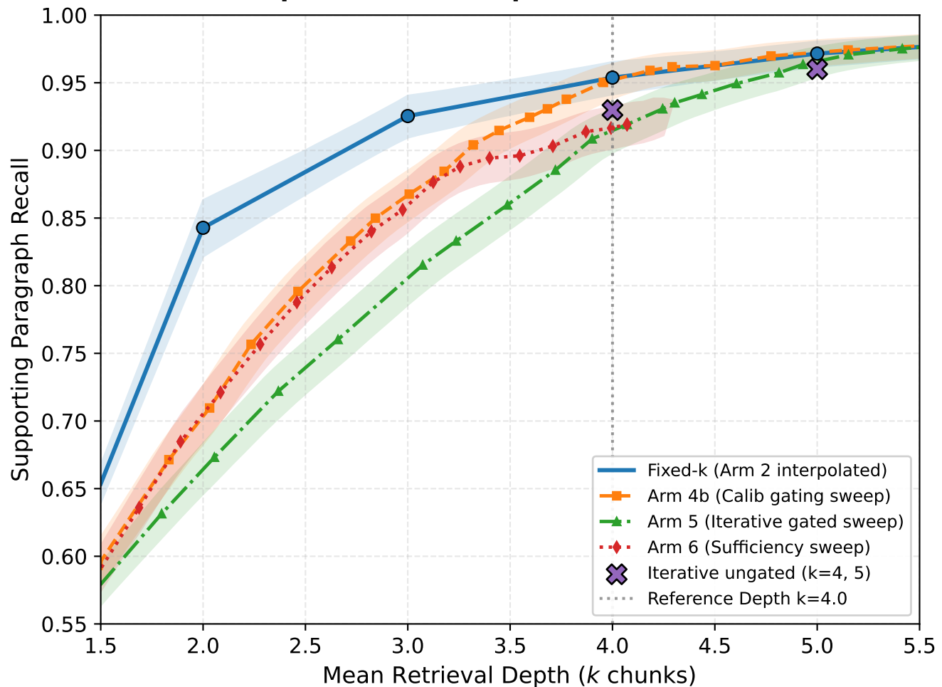
Comparison Multi-Hop Questions (N=563)
