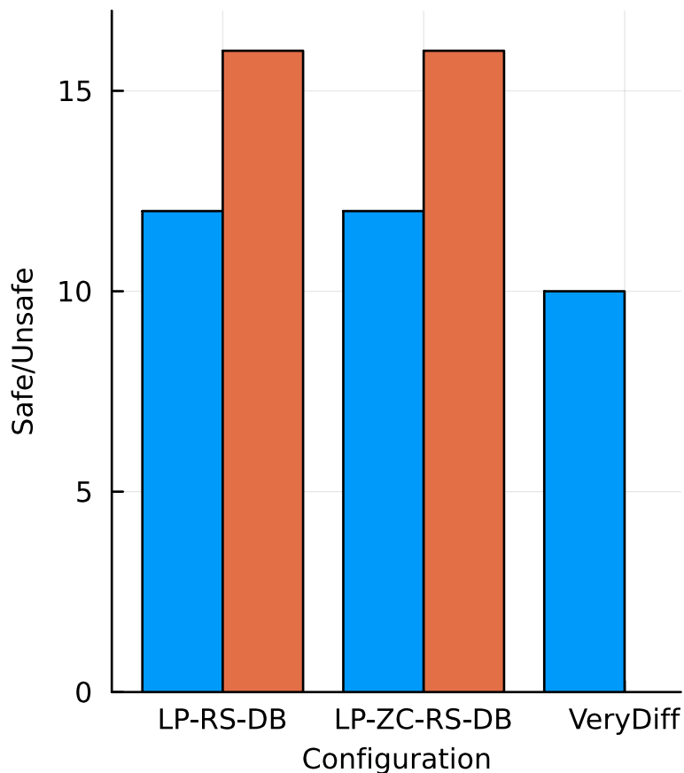
Neuron Splitting
