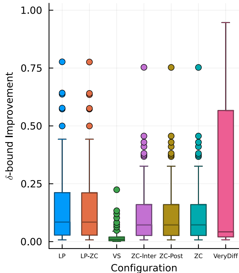
Neuron Splitting
