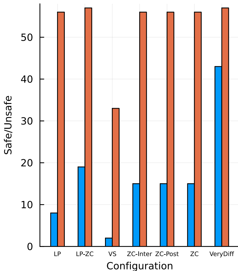
Neuron Splitting
