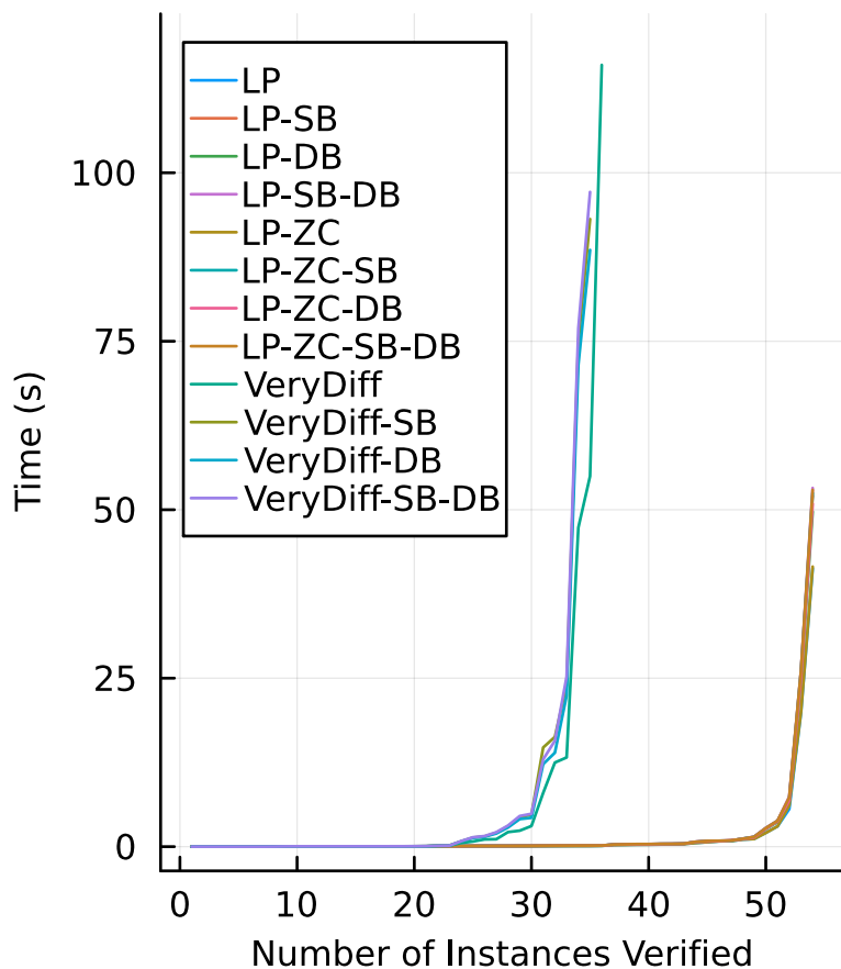
Neuron Splitting
