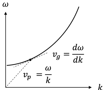
Figure 2.1: Illustration of phase velocity and group velocity.
