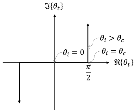
Figure 2.3: Illustration of the complex \theta_t plane.
