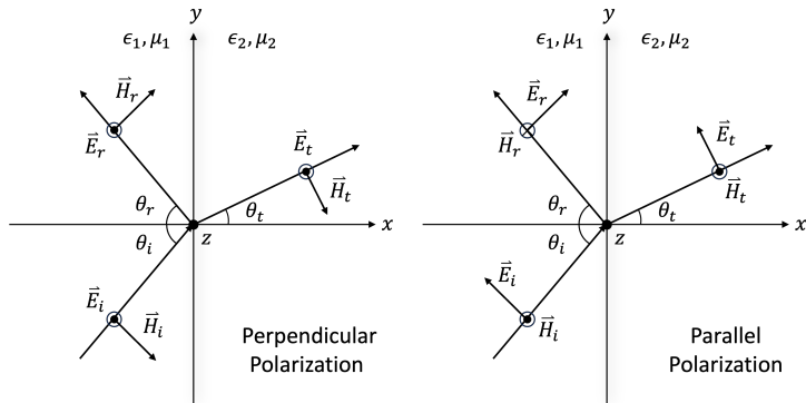
Figure 2.2: Illustration of the plane wave incident upon a plane interface with (i) perpendicular and (ii) parallel polarization.
