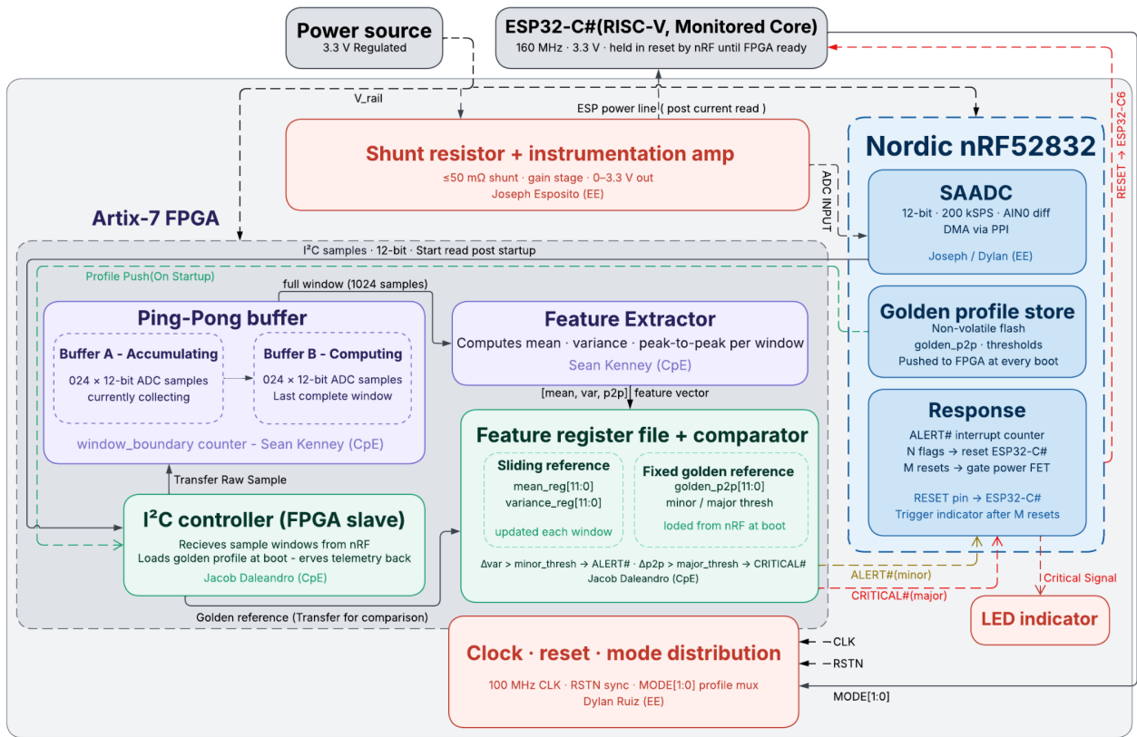
Figure 7.1: Hardware Block Diagram
