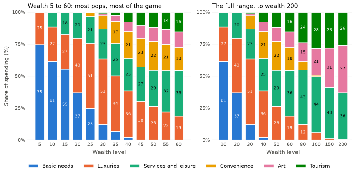
Figure 4: How a pop's spending divides between needs as its wealth rises, at base prices. Left: wealth 5 to 60, where most pops spend most of a campaign. Right: the full range to 200.
