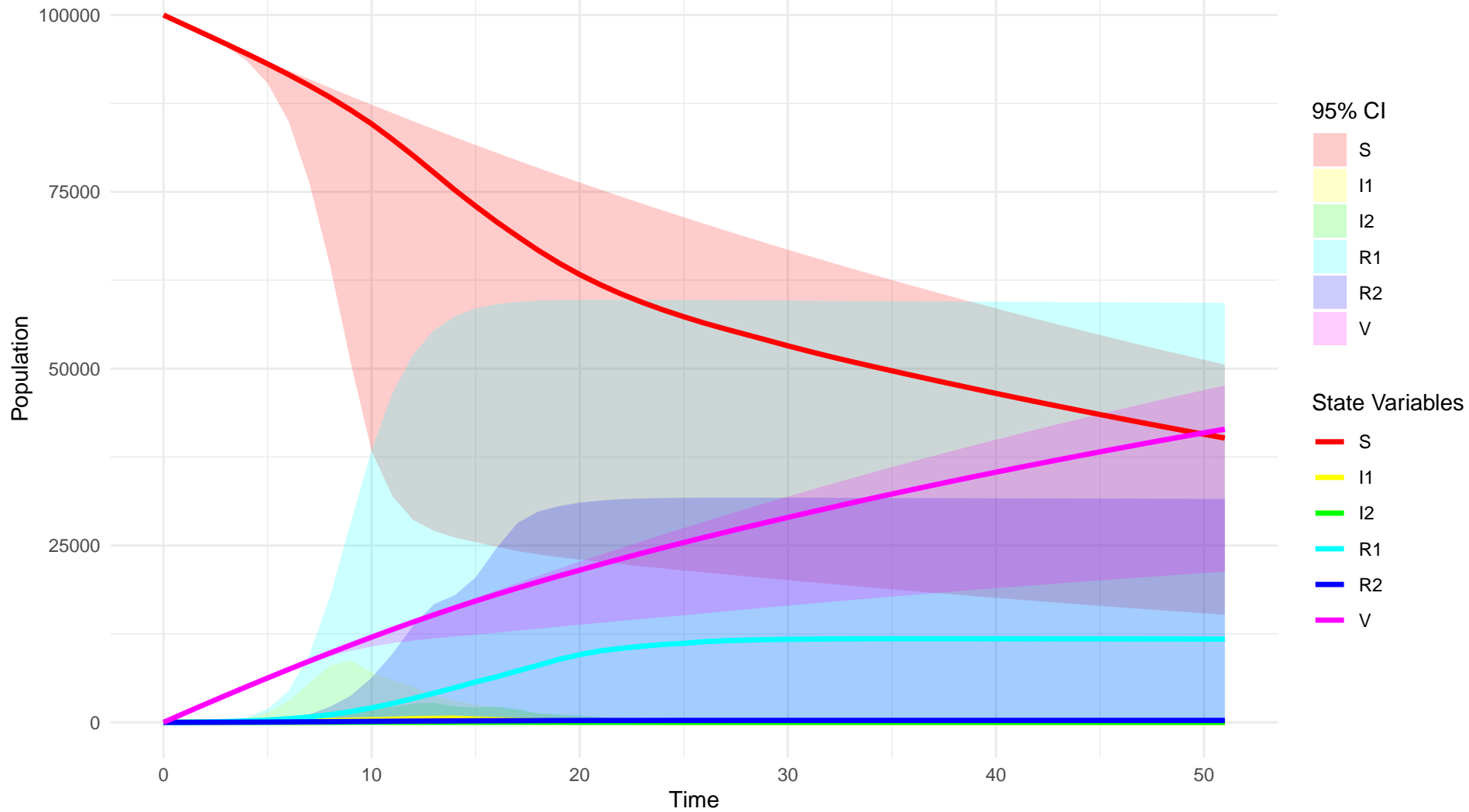
All ODE State Variables with Prior Uncertainty (95% CI)
