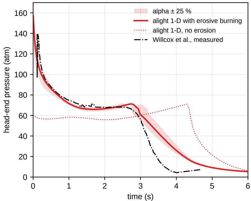
NAWC motor no. 6: head-end pressure
