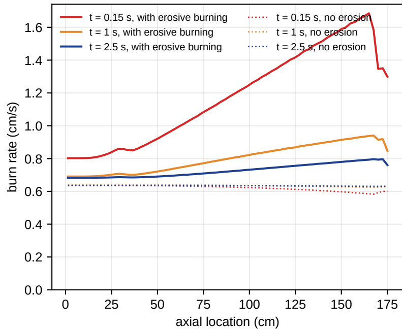
Burn rate along the port
