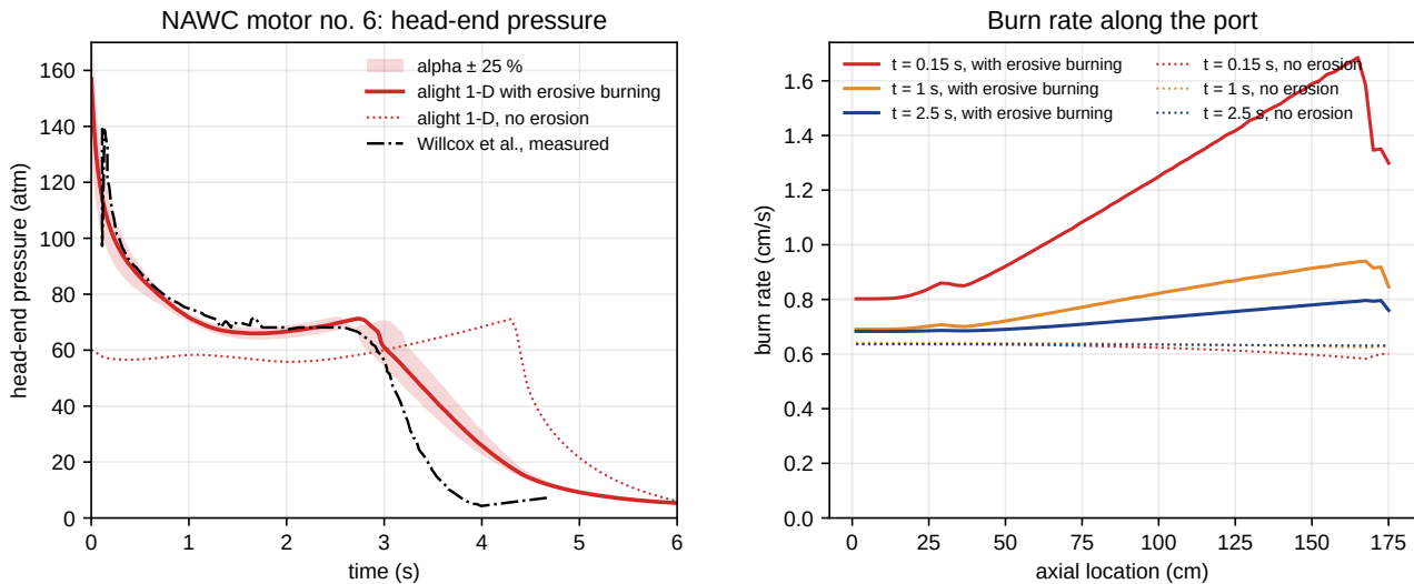
Figure 7: NAWC motor no. 6 with the 1-D model. Left: head-end pressure with and without erosive burning against the measured trace; the band is \alpha \pm 25\% . Right: burn rate along the port at three times.
