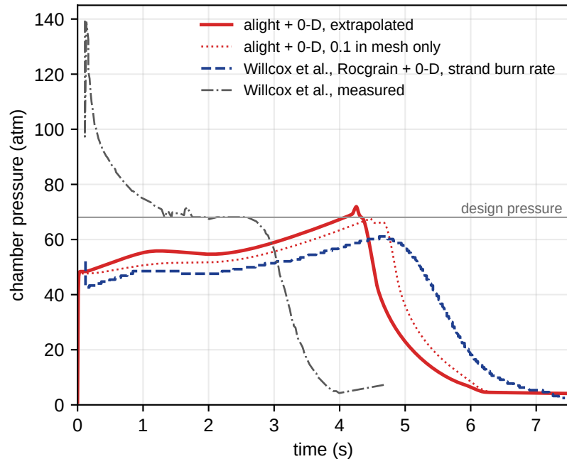
Chamber pressure
