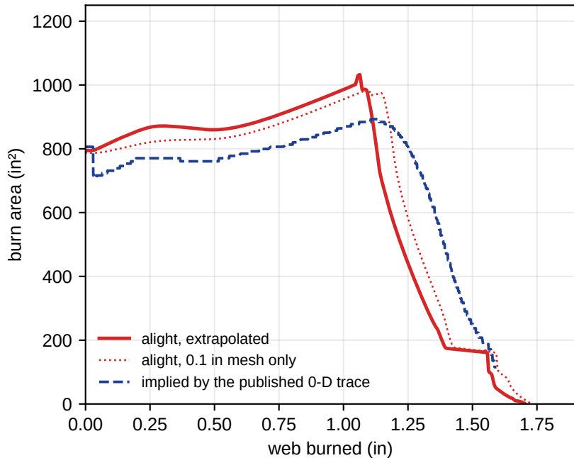
NAWC motor no. 6: burn area
