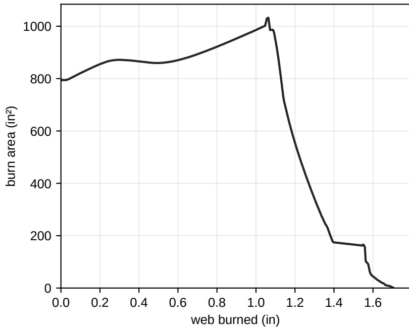
NAWC motor no. 6: burn area from alight
