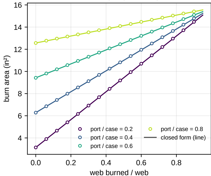
Tube, ends inhibited: alight (markers) and closed form
