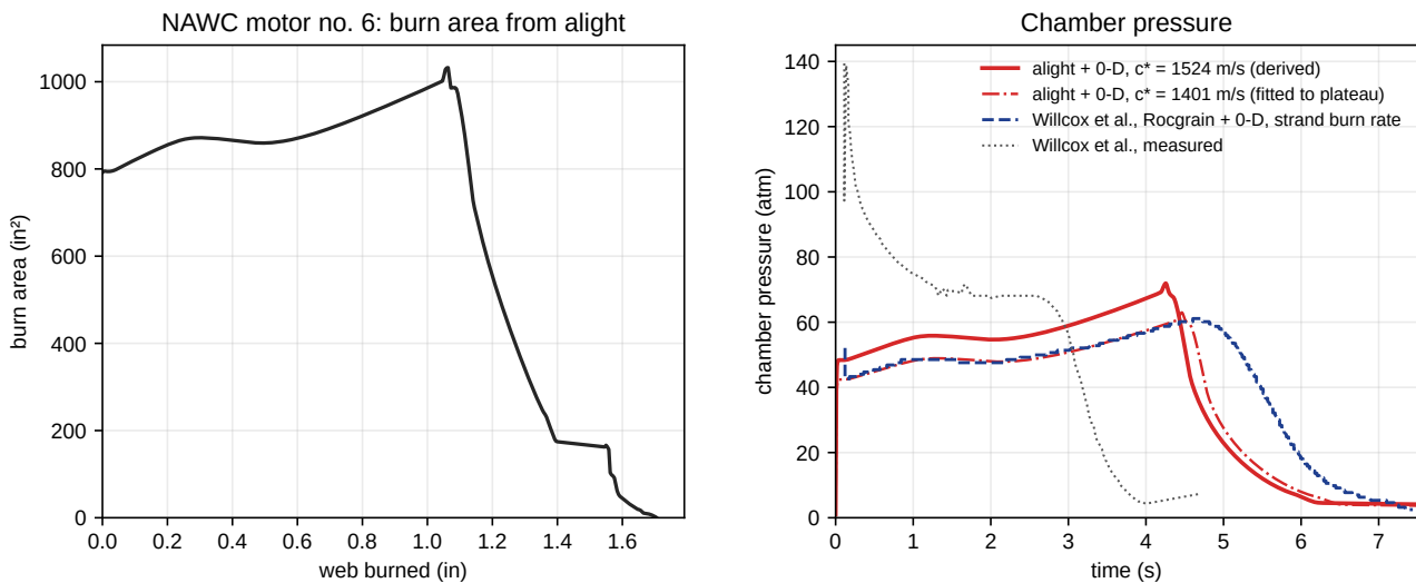
Figure 6: NAWC motor no. 6. Left: burn area from alight. Right: chamber pressure from alight with 0-D ballistics, the published 0-D simulation with the strand burn rate, and the measured trace.
