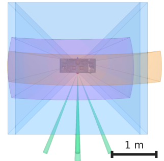
Bow-on — DVL beams
