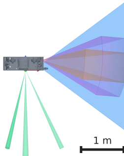
Starboard — elevation
