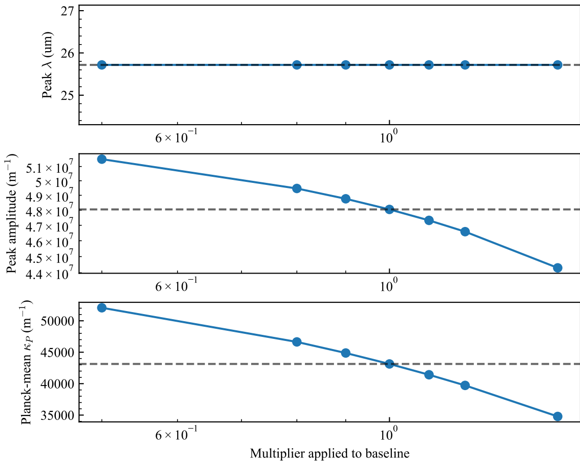
Sensitivity: epsilon_inf (baseline=1.96)
