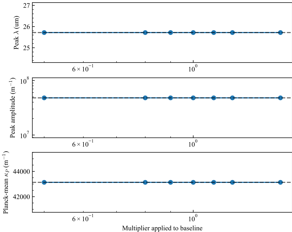
Sensitivity: kappa0 (baseline=1e+08)
