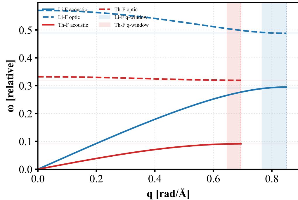
Li-F vs Th-F — S = 0.000
