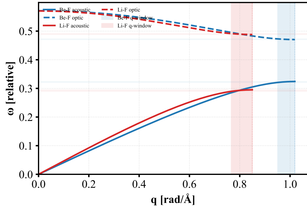
Be-F vs Li-F — S = 0.000
