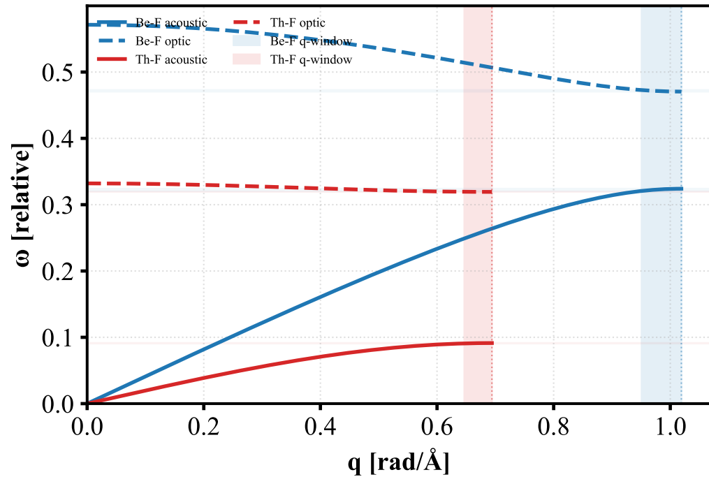
Be-F vs Th-F — S = 0.000
