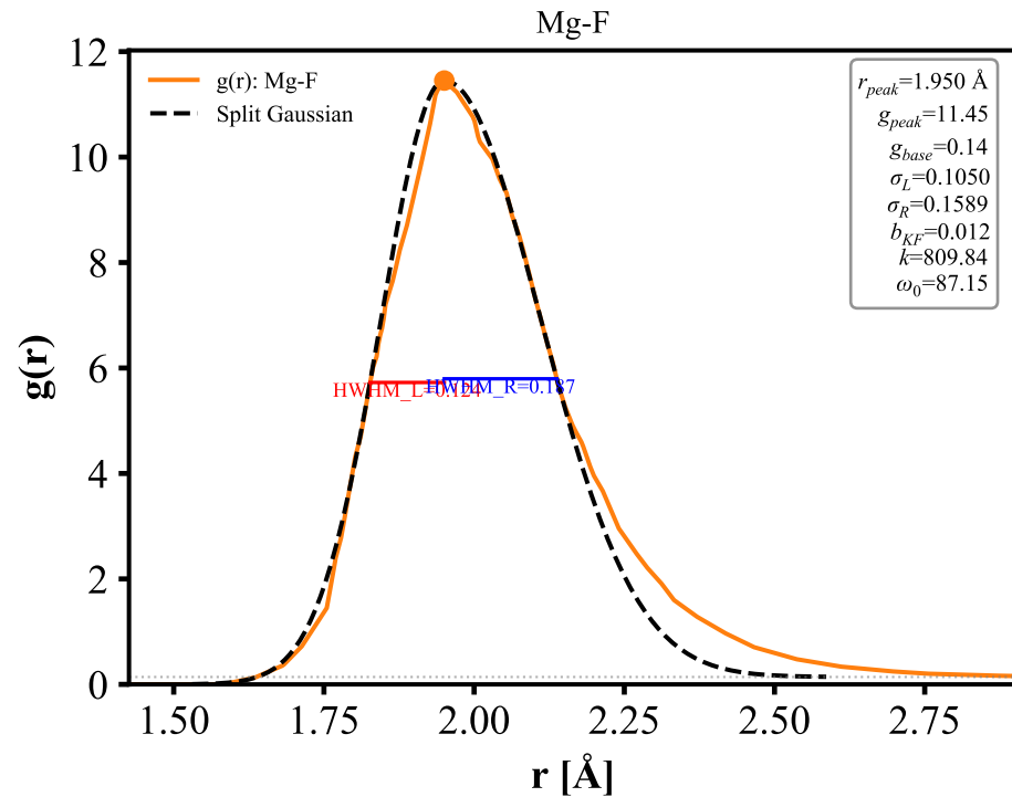
0.345NaF-0.065MgF 2 -0.59KF (1073K) — Split Gaussian
