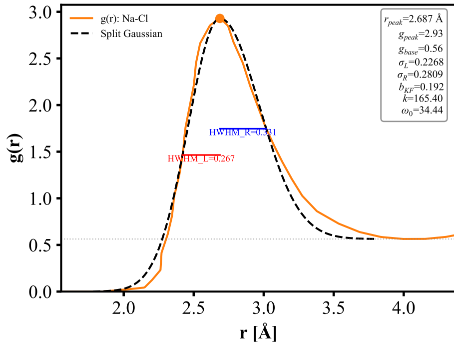
Na-Cl
