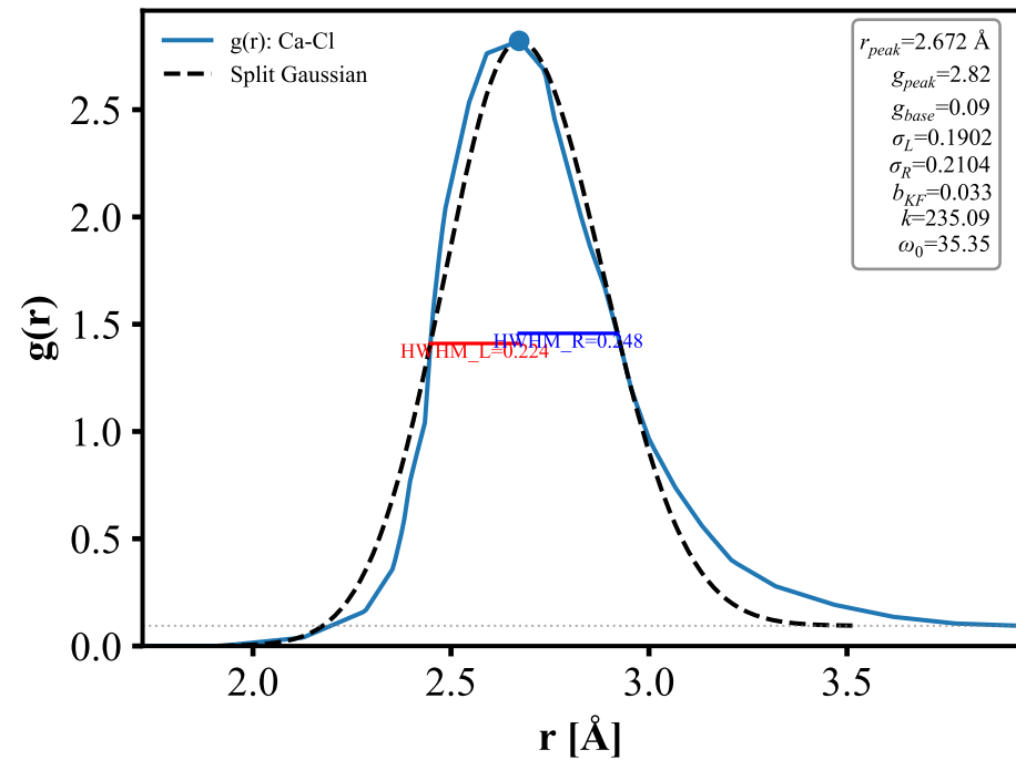
Ca-Cl
