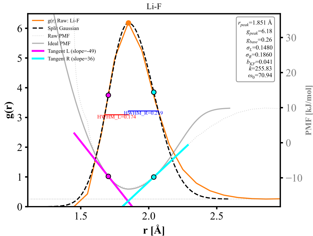
0.465LiF-0.115NaF-0.42KF (873K) — Analytical Inflection & PMF
