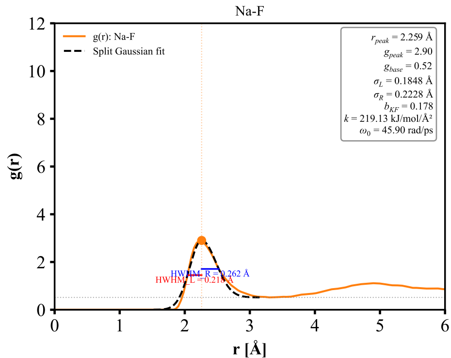
0.57NaF-0.16KF-0.27UF 4 (900K) — Split Gaussian Fits
