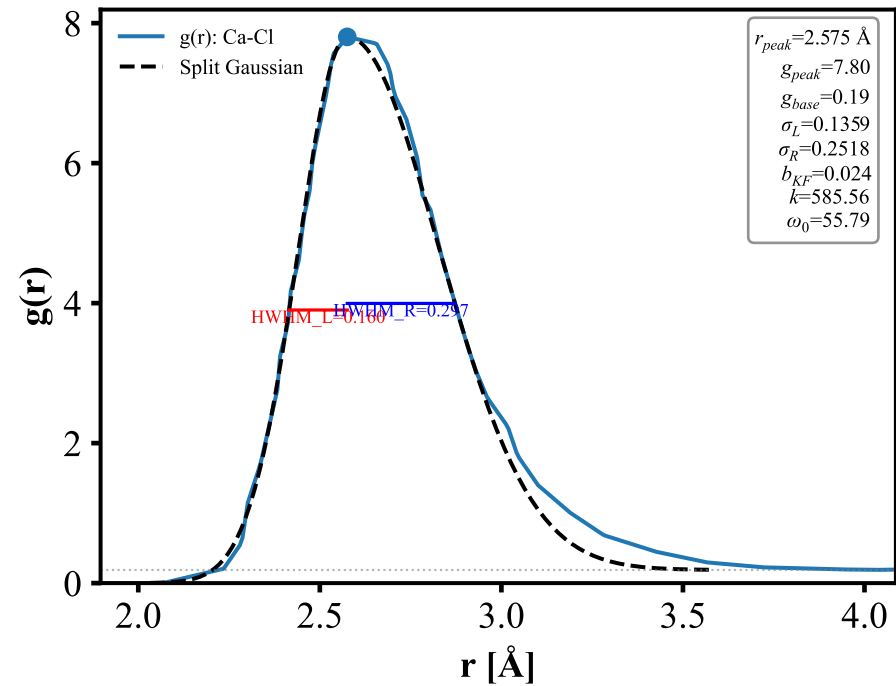
Ca-Cl
