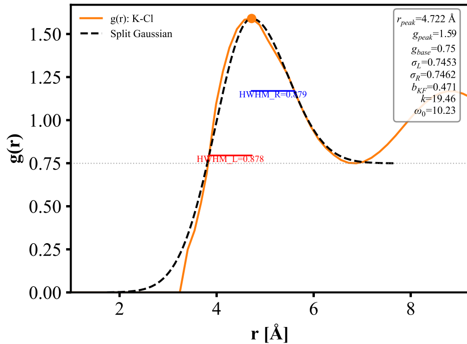
K-Cl
