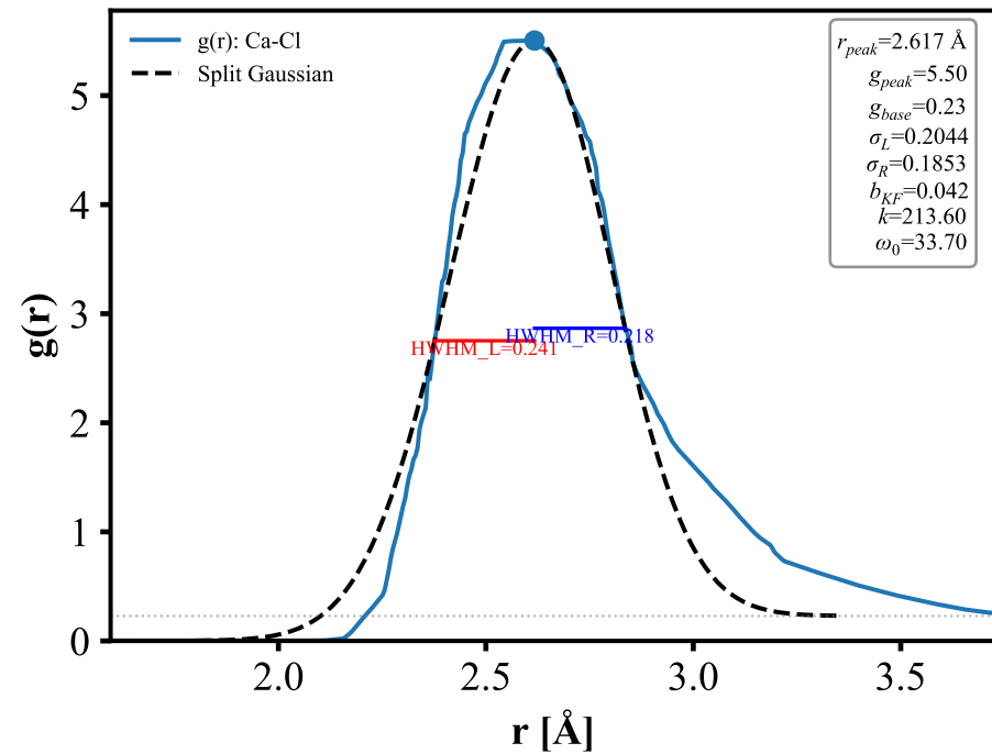
Ca-Cl
