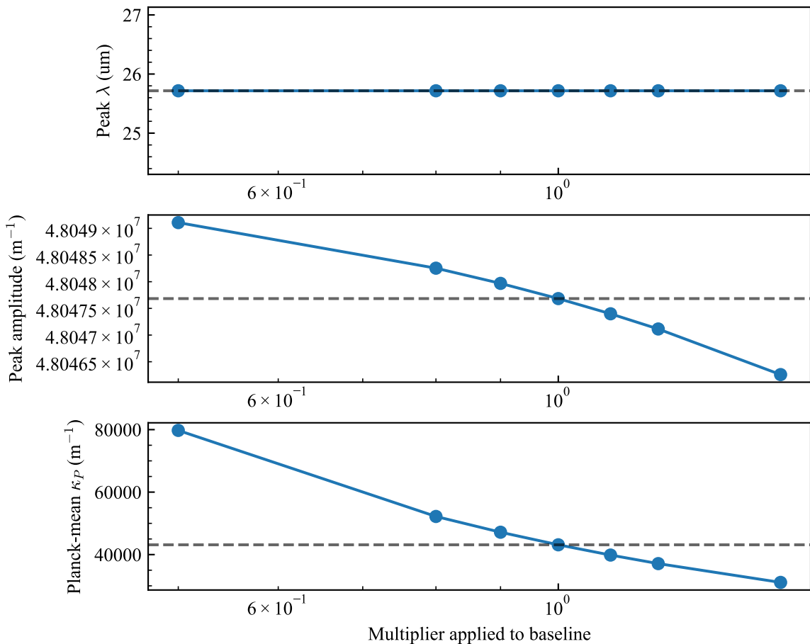
Sensitivity: eps_inf_mixture (baseline=1.96)
