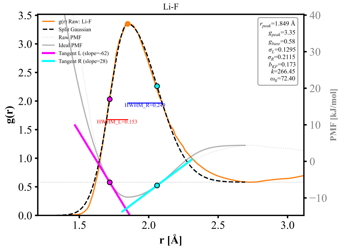
0.6LiF-0.3BeF 2 -0.1ThF 4 (973K) — Analytical Inflection & PMF
