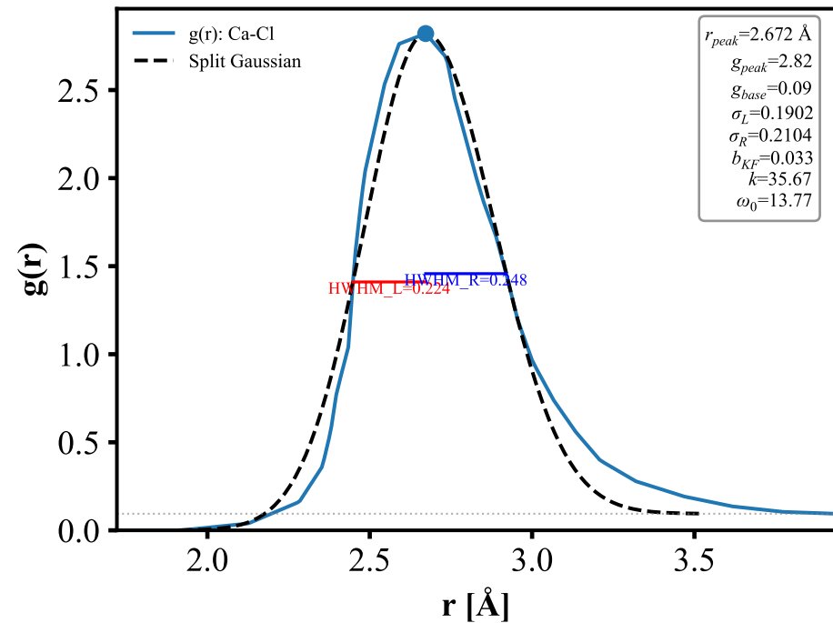
Ca-Cl
