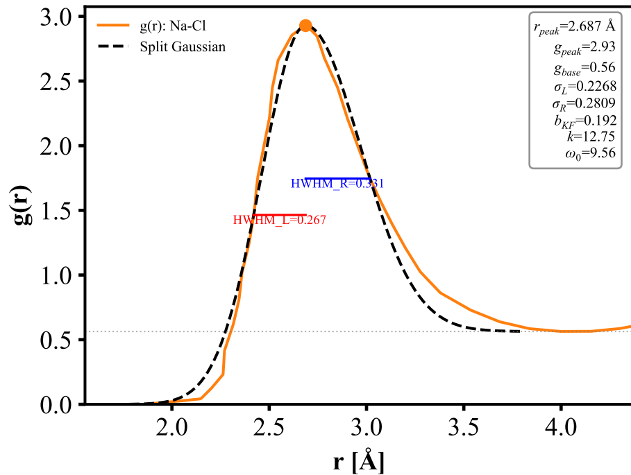
Na-Cl
