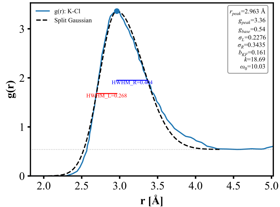
K-Cl
