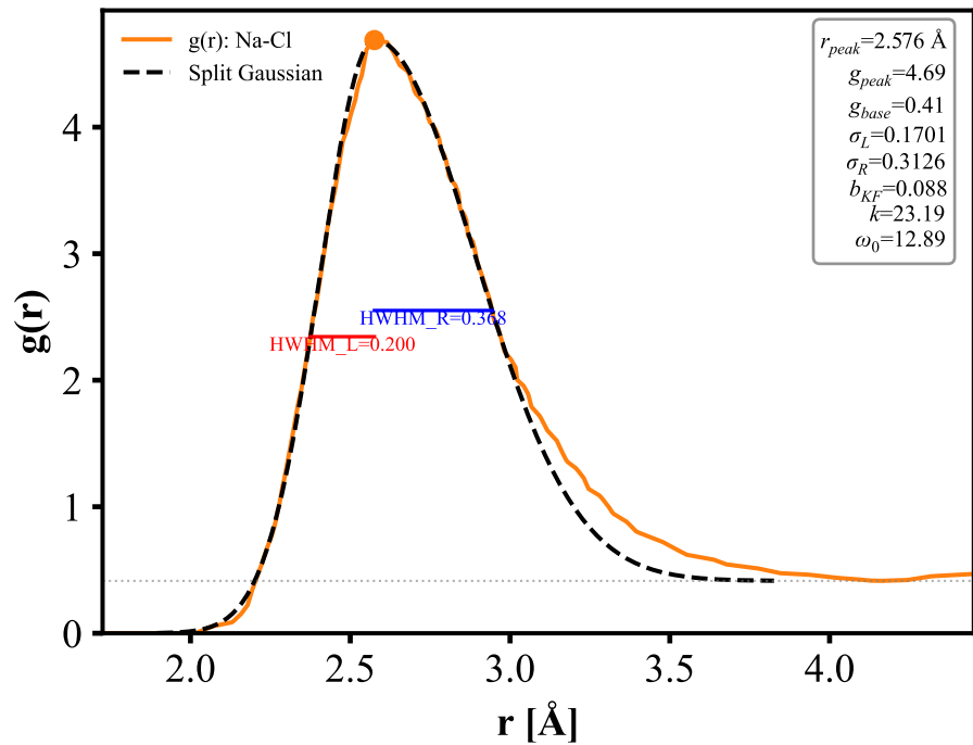
Na-Cl
