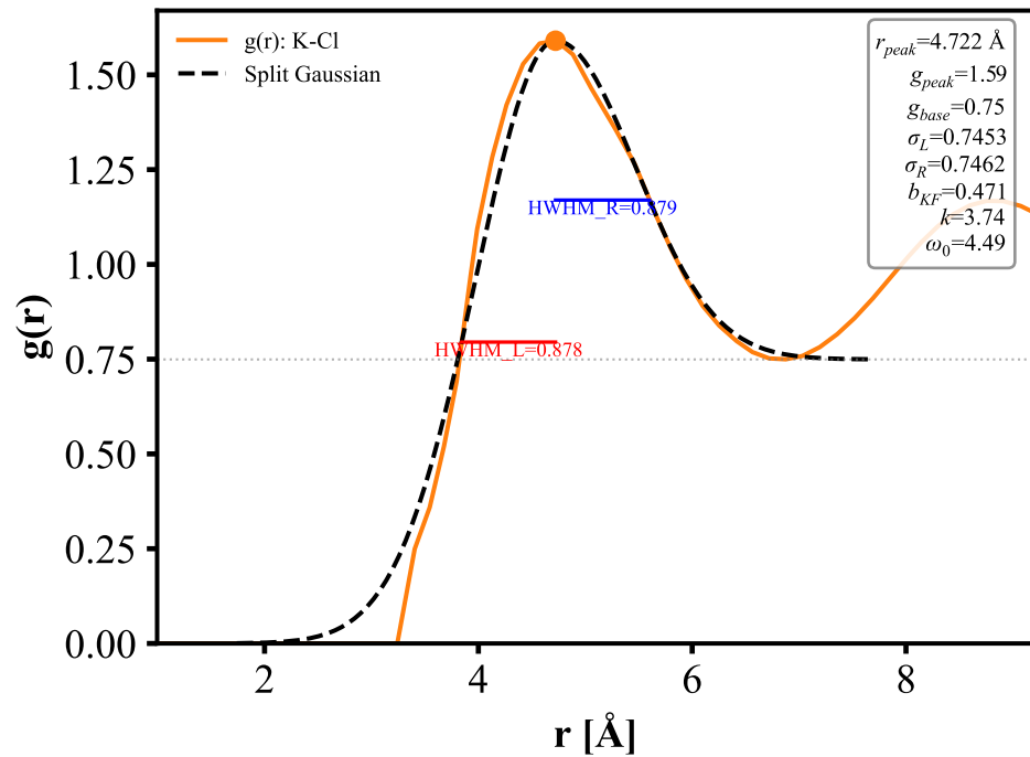
K-Cl
