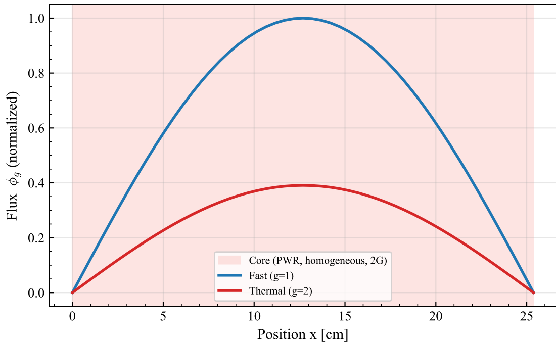
Case 1 - Bare PWR (w = 25.38 cm, k = 0.99999)
