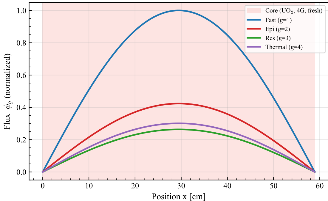
Case 1b - Bare PWR 4-group (w = 58.93 cm, k = 1.00000)
