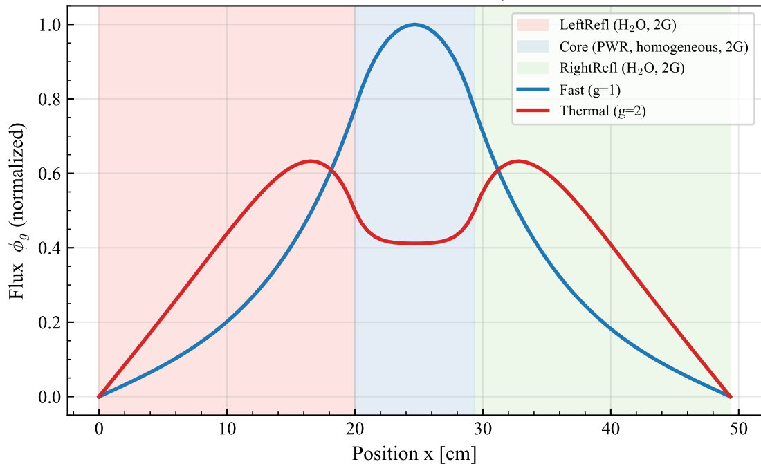
Case 2 - Reflected PWR ( w_{core} = 9.34 cm, w_{ref} = 20.00 cm, k = 1.00001 )
