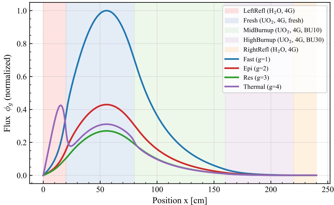
Case 3 - 5-region 4-group core (k = 1.10128)
