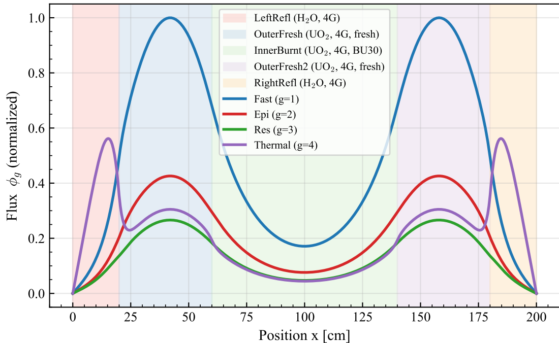
Case 3b - Flat-flux core ( k = 1.04041 )
