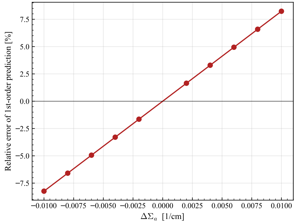
Case 4 - Rayleigh validation: PWR thermal absorption - error
