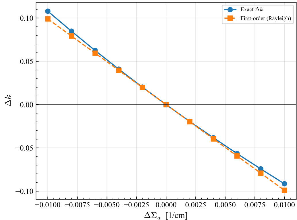
Case 4 - Rayleigh validation: PWR thermal absorption
