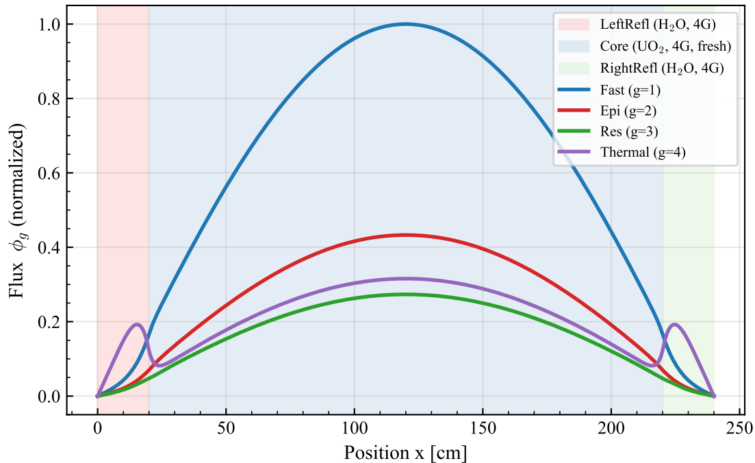
Case 5 - 4-group UO 2 + H 2 O ( k = 1.15637 )
